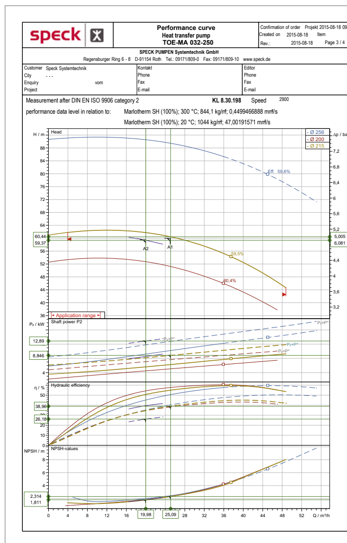
Characteristic curve (example)
